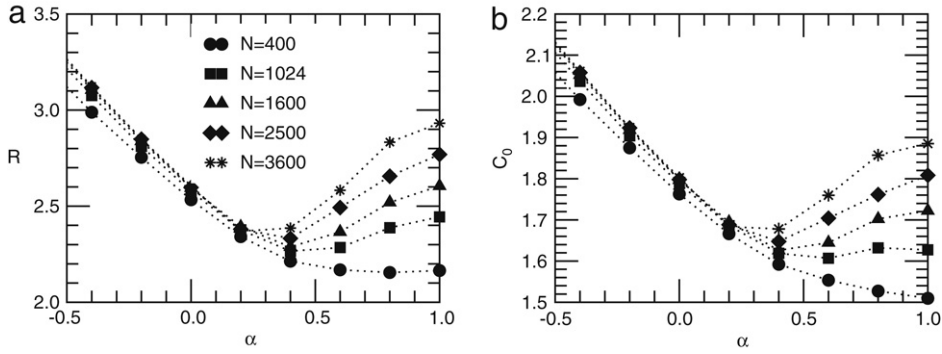
Fig. 25. Eigenratio R (a) and normalized cost C_0 (b) as a function of the parameter \alpha in Eq. (100), for random SF networks with \gamma = 3 and k_{\min} = 10 . From [149].
